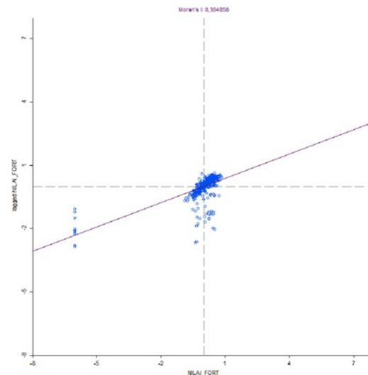
Fig. 4 Scatter plot Moran's I.
