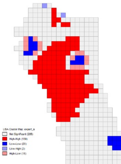
Fig. 6 LISA Cluster Map
