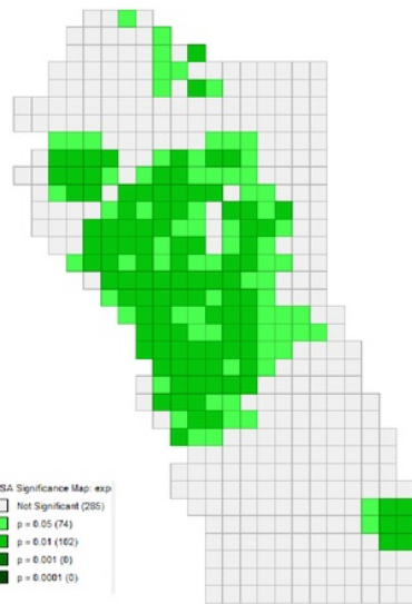
Fig. 5 LISA Significant Map
